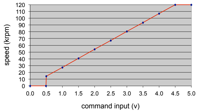
S24V5A - 3F command input vs speed
