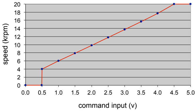
S24V5A - 3C command input vs speed
