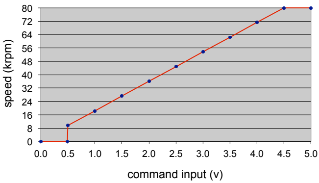
S24V5A - 4E command input vs speed
