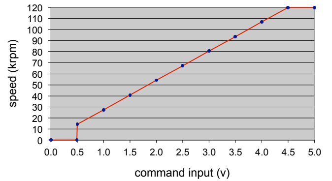
S24V5A - 4F command input vs speed
