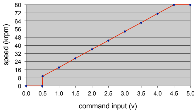
S24V5A - 3E command input vs speed
