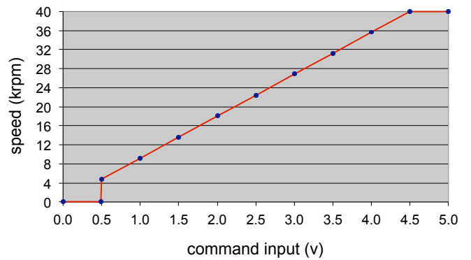
S24V5A - 4D command input vs speed
