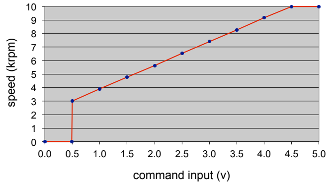
S24V5A - 4B command input vs speed
