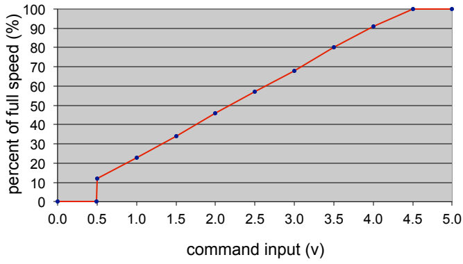
S24V5A - 3A command input vs percent of full speed
