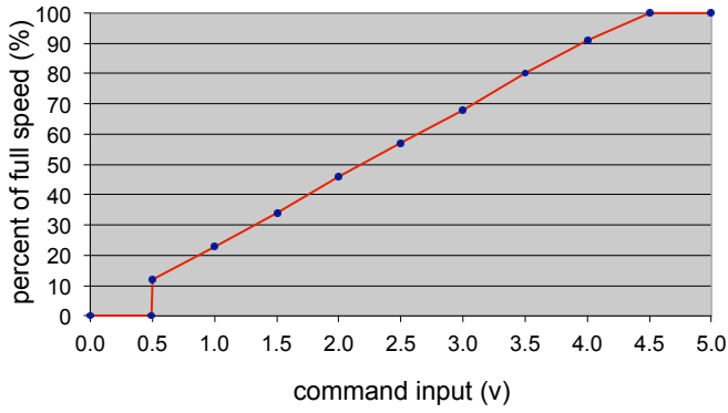
S24V5A - 4A command input vs percent of full speed
