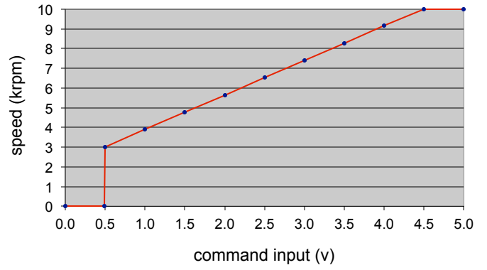
S24V5A - 3B command input vs speed
