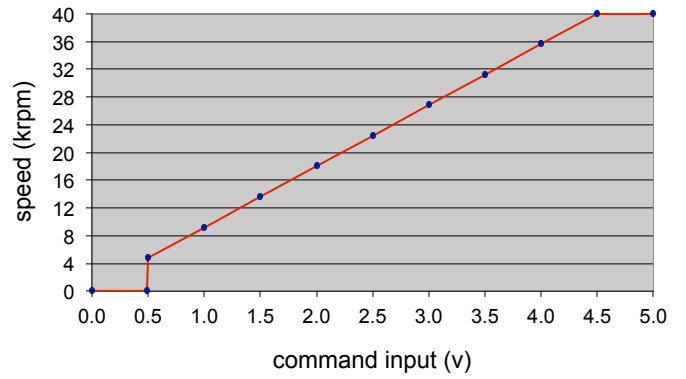
S24V5A - 3D command input vs speed
